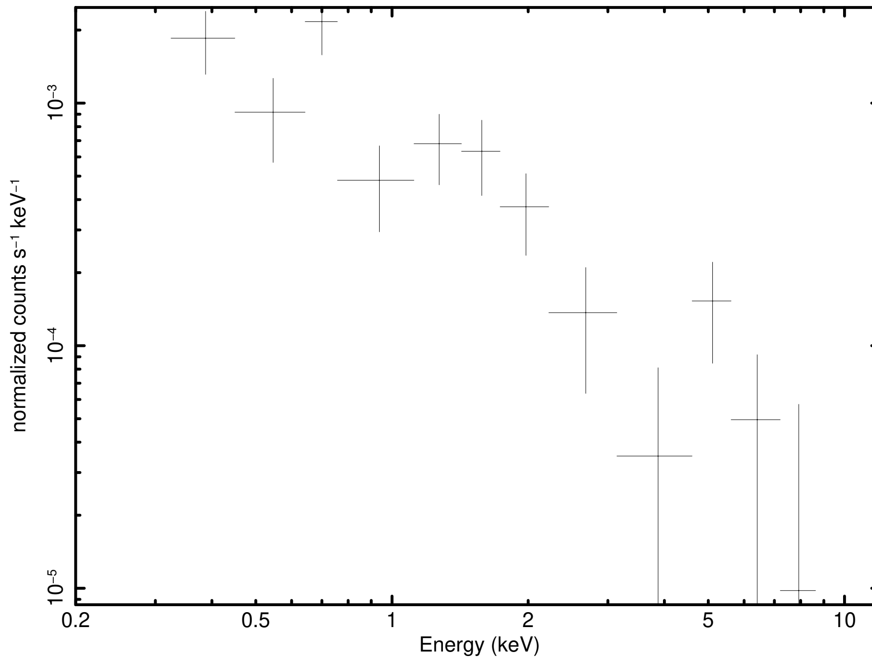
Source 78 minus background (P0931790101PNS003SRSPEC004E)
