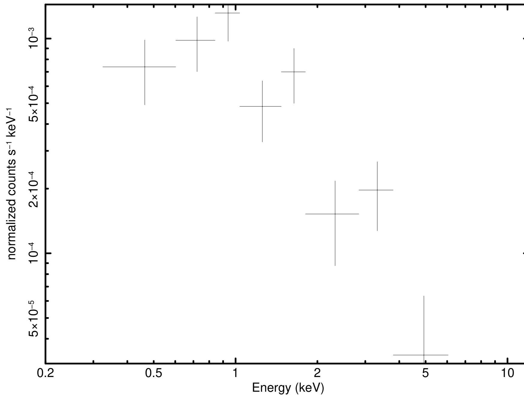
Source 80 minus background (P0931790101PNS003SRSPEC0050)
