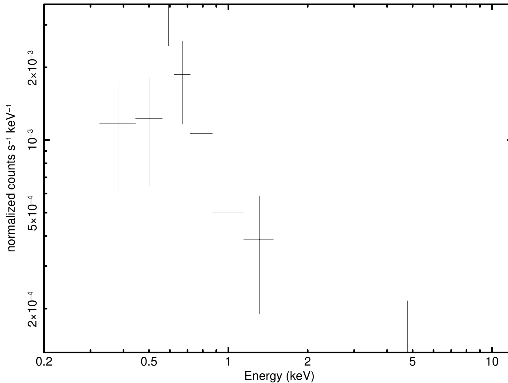
Source 81 minus background (P0931790101PNS003SRSPEC0051)
