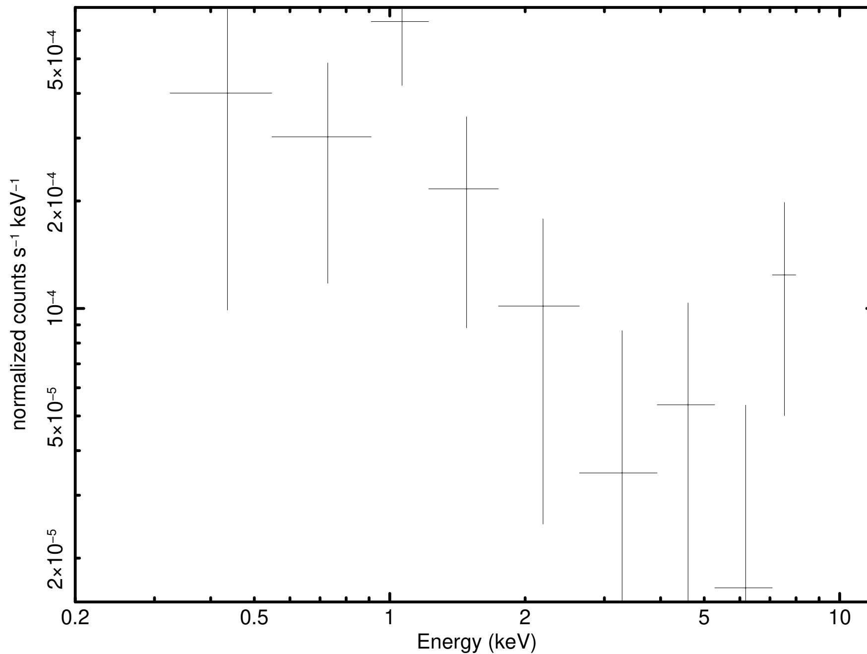
Source 84 minus background (P0931790101PNS003SRSPEC0054)
