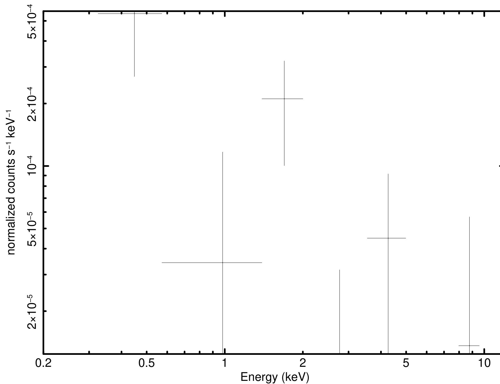
Source 86 minus background (P0931790101PNS003SRSPEC0056)
