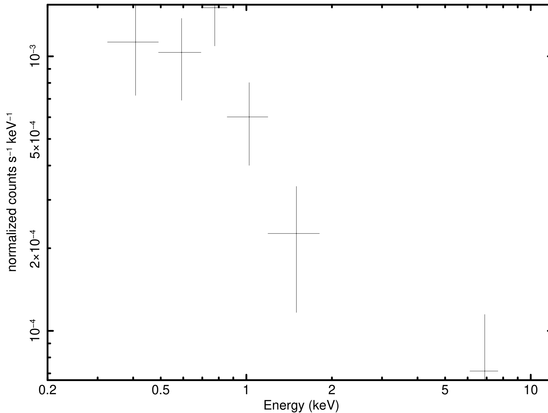
Source 87 minus background (P0931790101PNS003SRSPEC0057)
