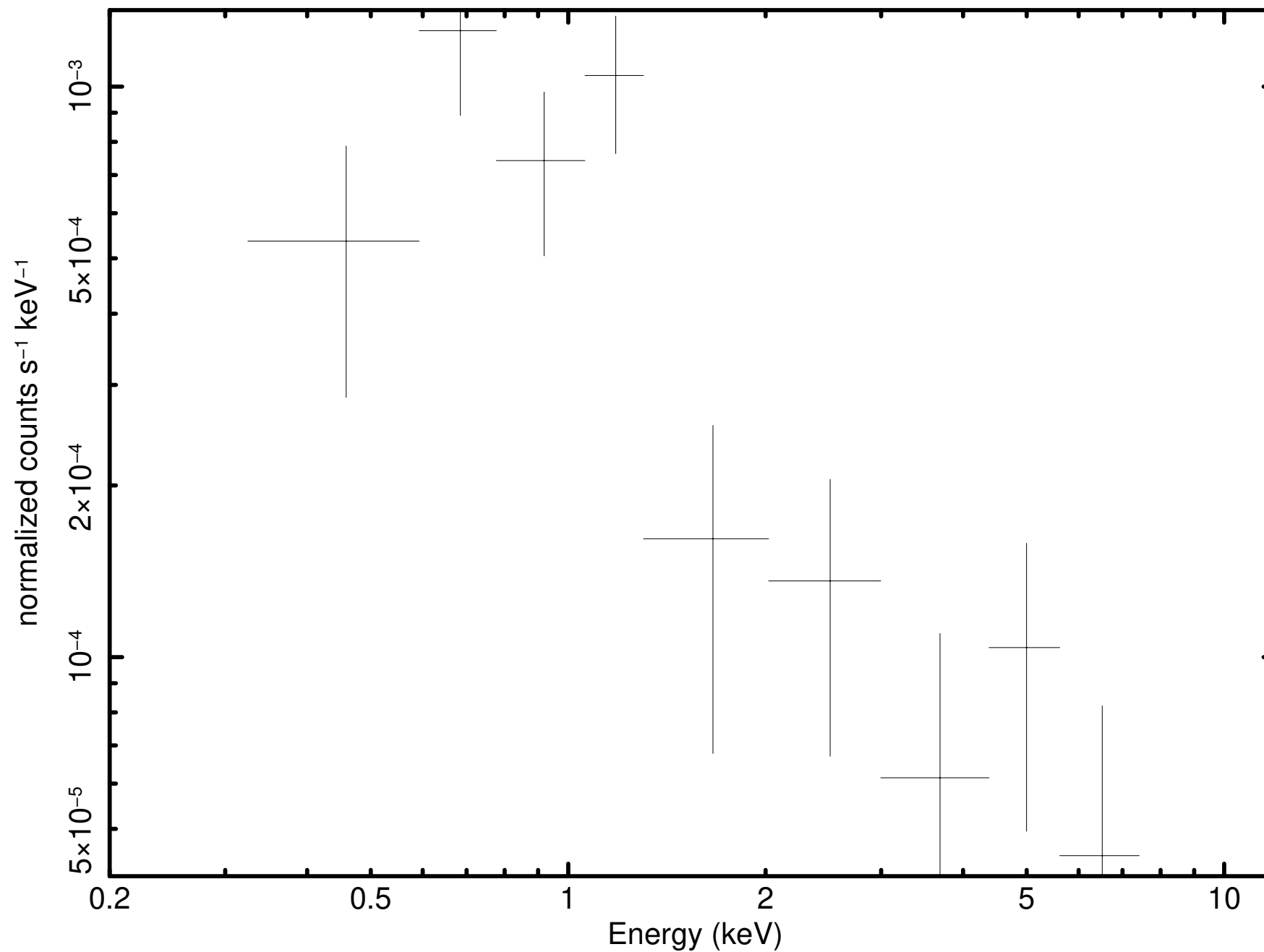
Source 88 minus background (P0931790101PNS003SRSPEC0058)
