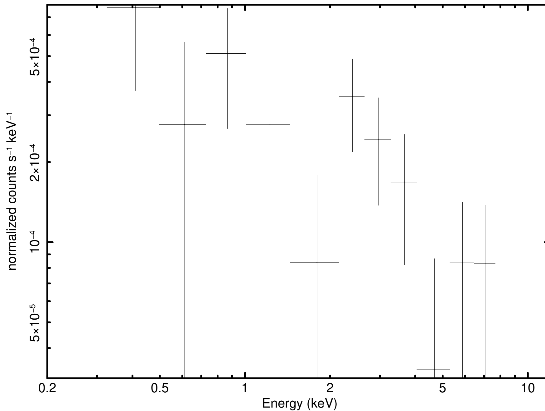
Source 90 minus background (P0931790101PNS003SRSPEC005A)
