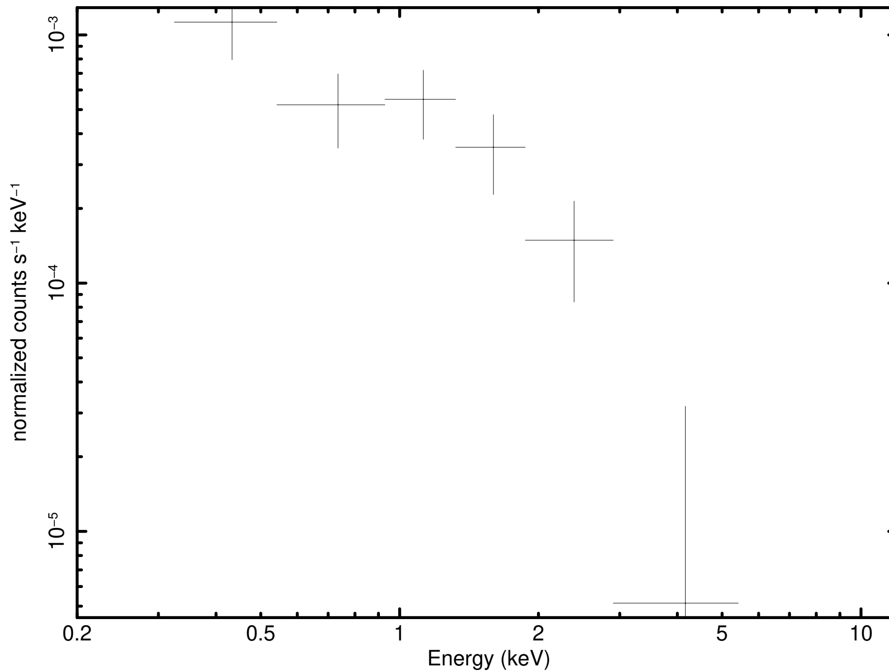
Source 91 minus background (P0931790101PNS003SRSPEC005B)
