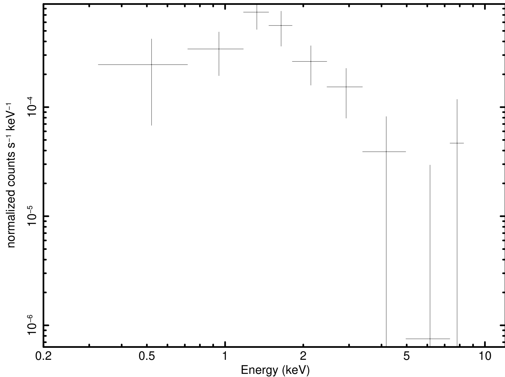
Source 93 minus background (P0931790101PNS003SRSPEC005D)
