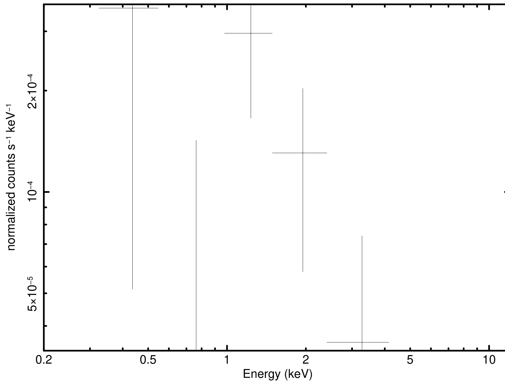
Source 94 minus background (P0931790101PNS003SRSPEC005E)
