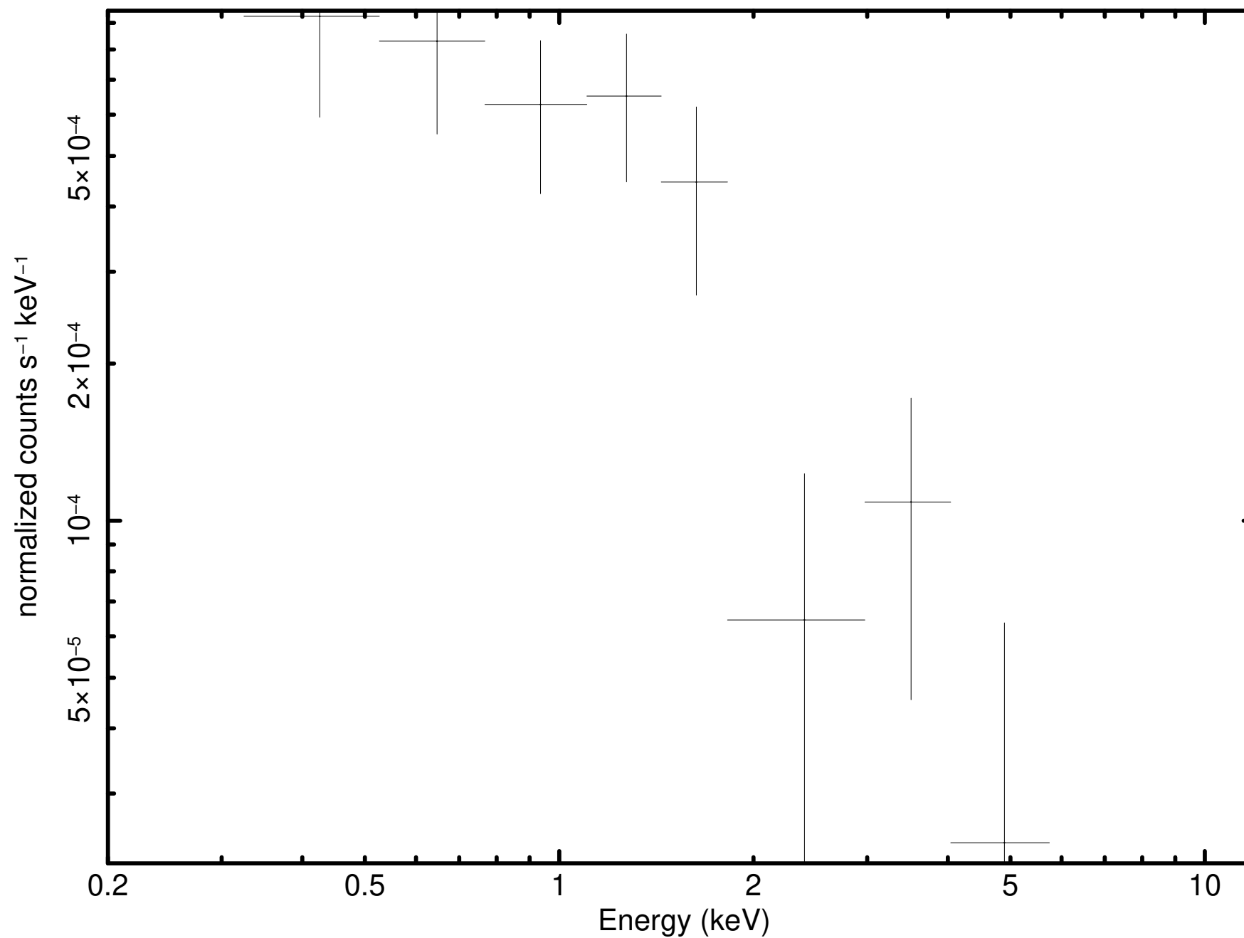
Source 96 minus background (P0931790101PNS003SRSPEC0060)
