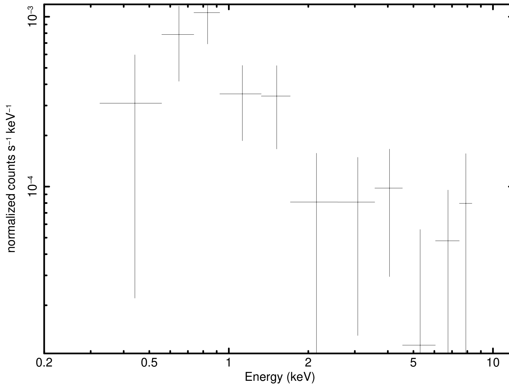
Source 97 minus background (P0931790101PNS003SRSPEC0061)
