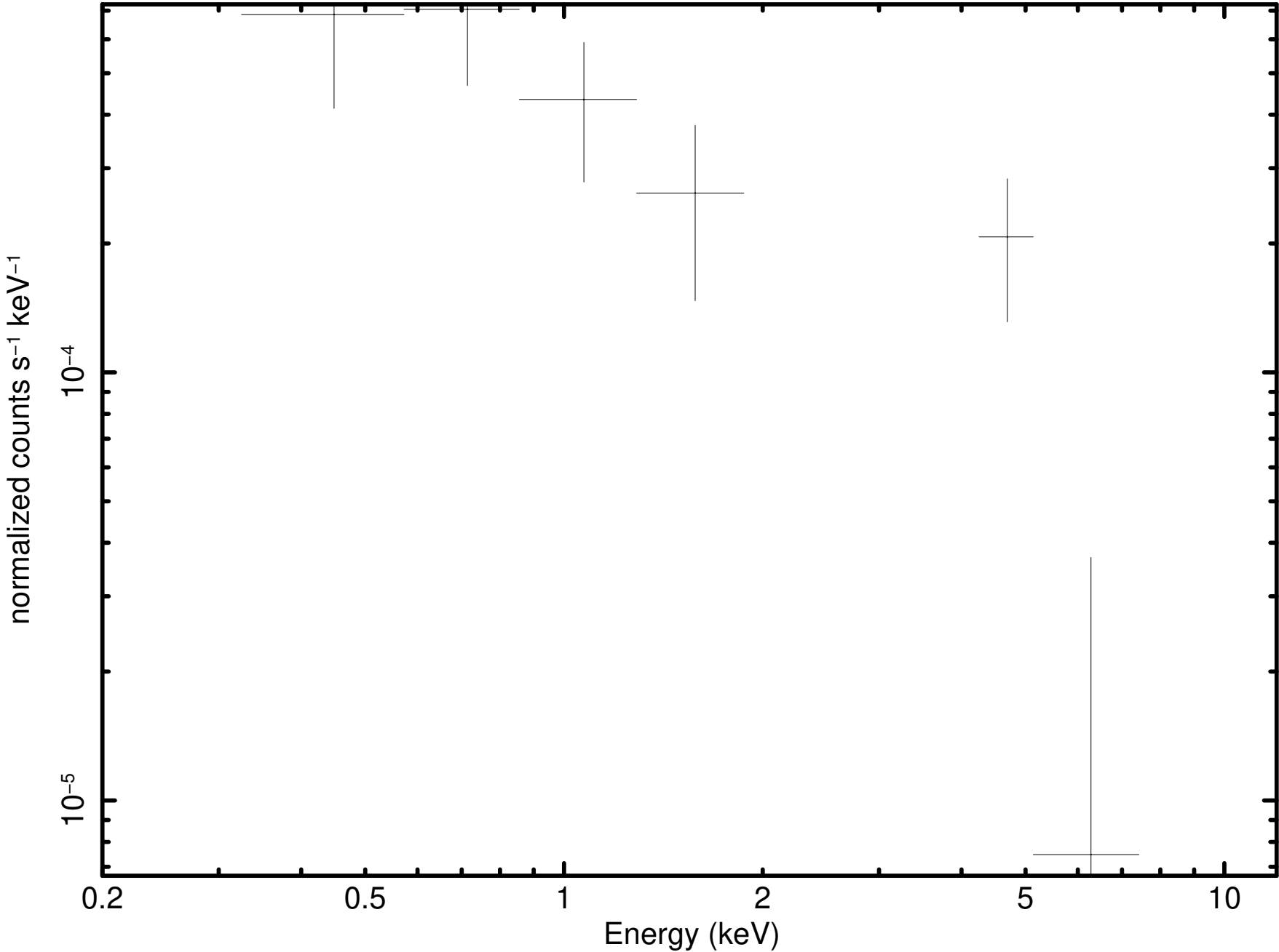
Source 102 minus background (P0931790101PNS003SRSPEC0066)
