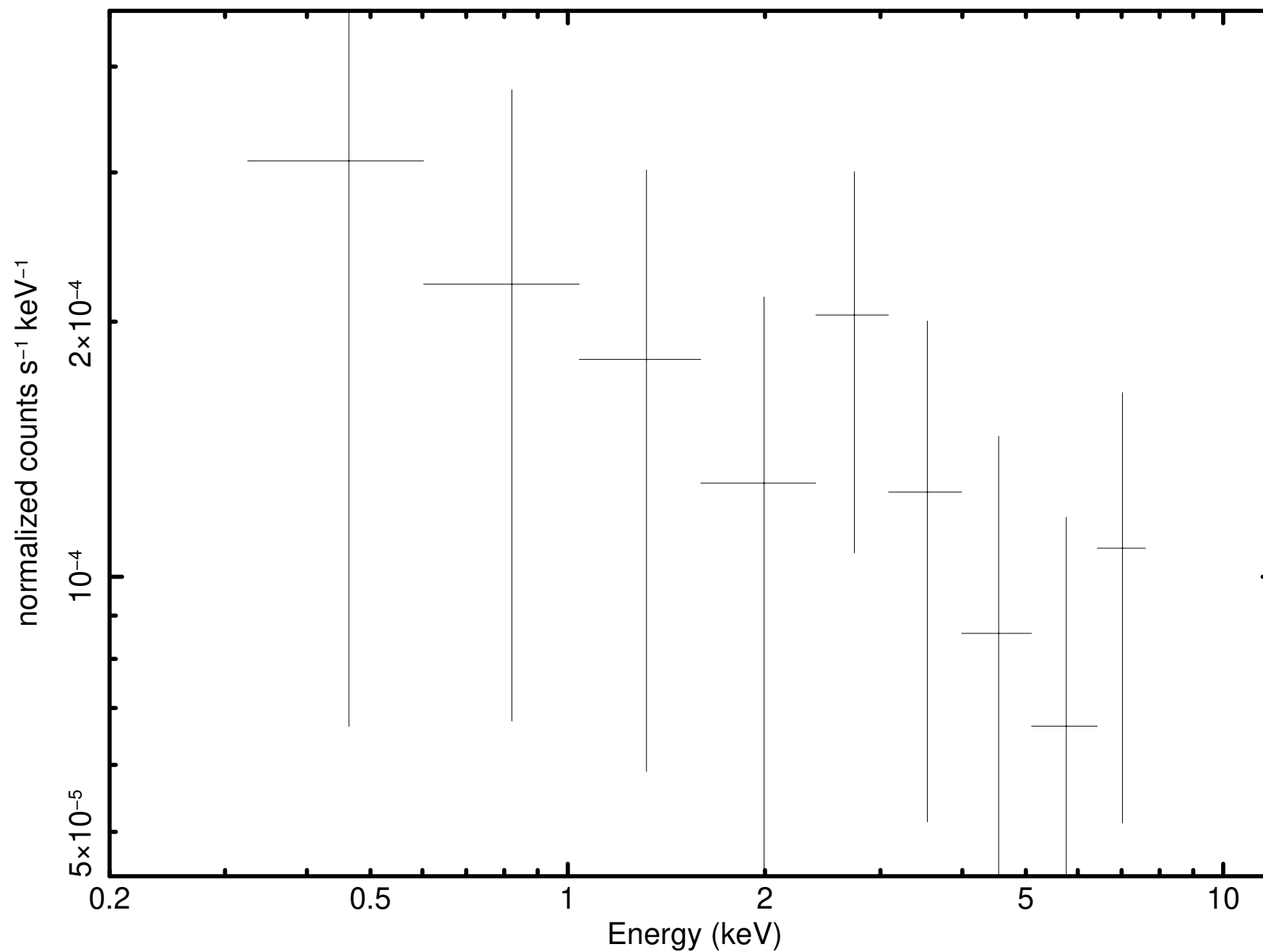
Source 103 minus background (P0931790101PNS003SRSPEC0067)
