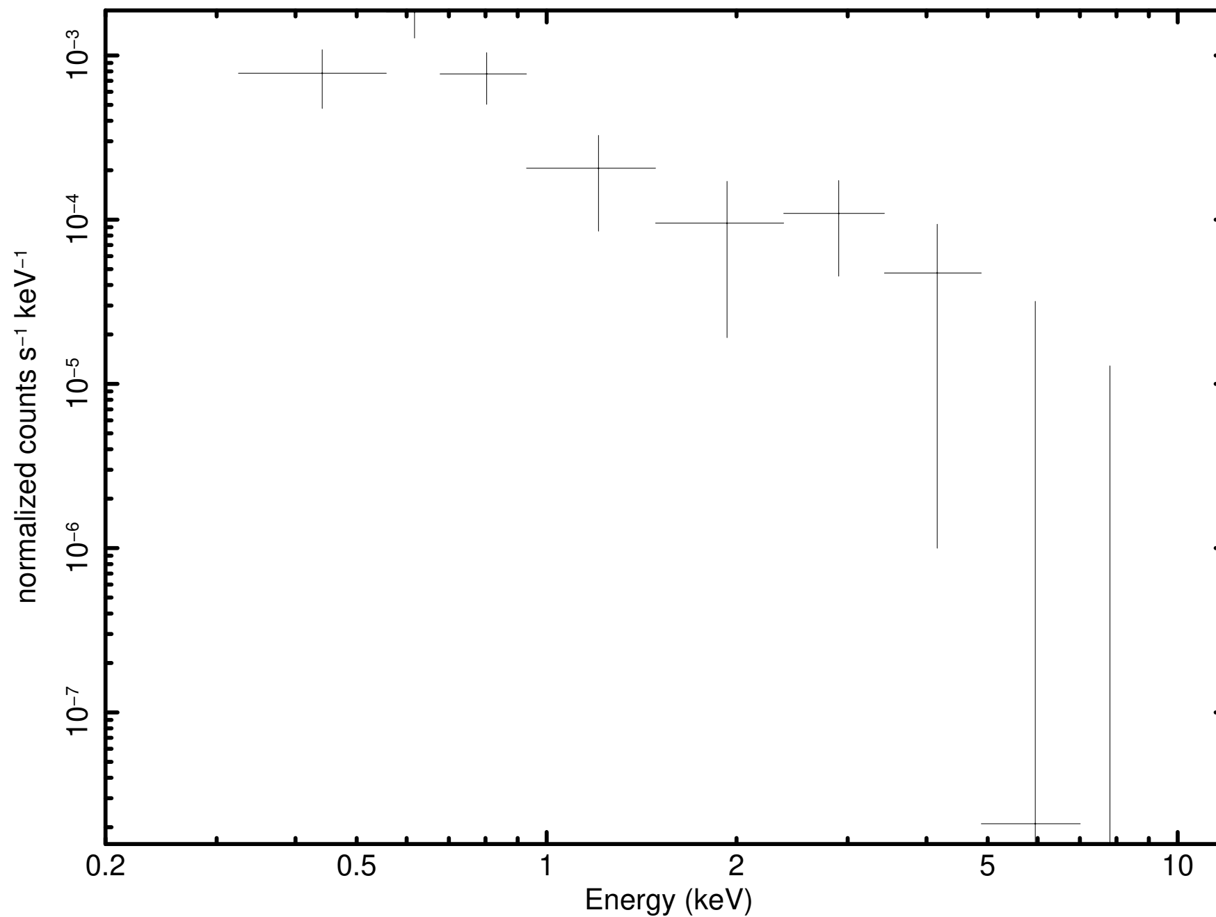
Source 107 minus background (P0931790101PNS003SRSPEC006B)
