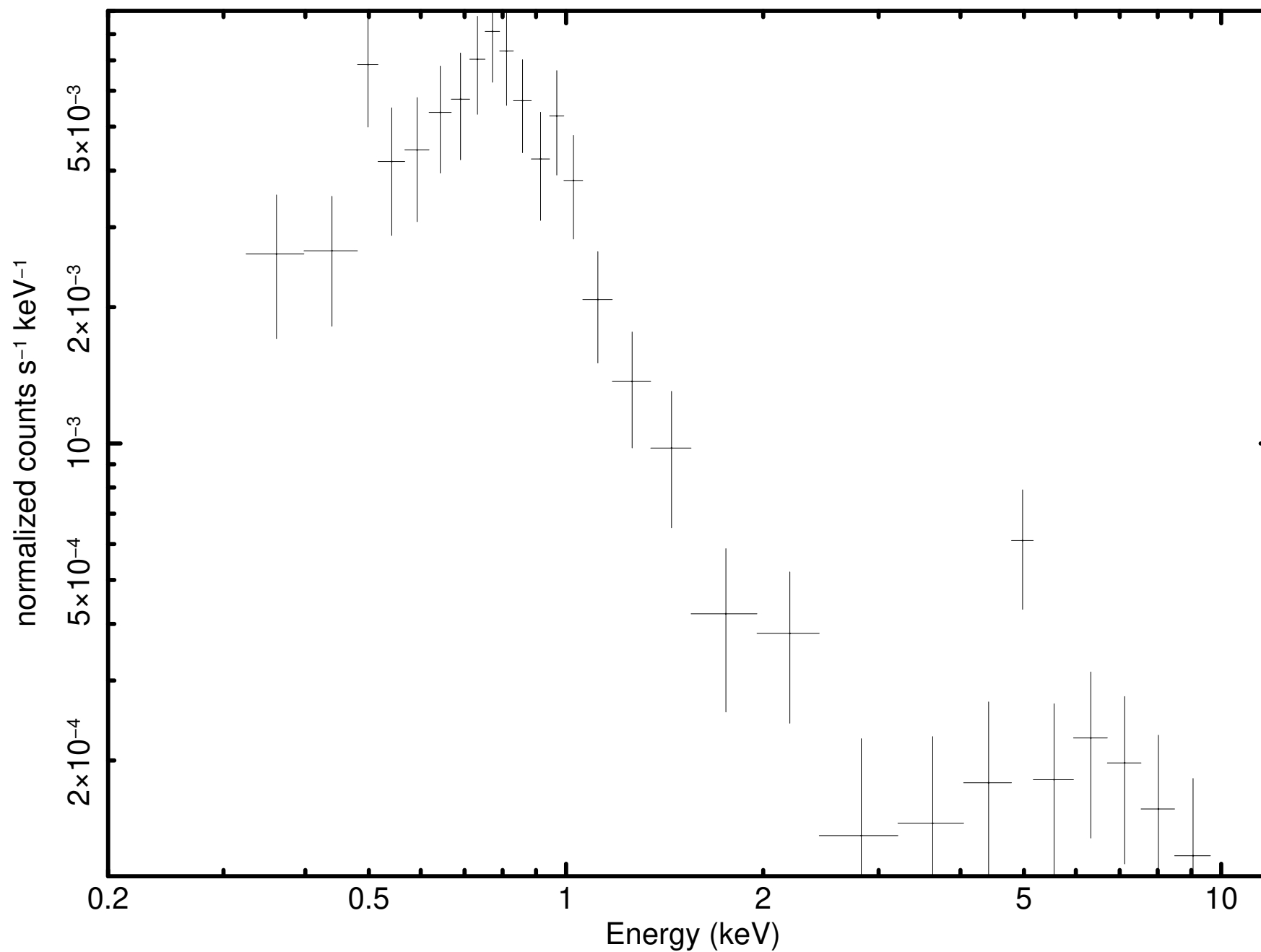
Source 109 minus background (P0931790101PNS003SRSPEC006D)
