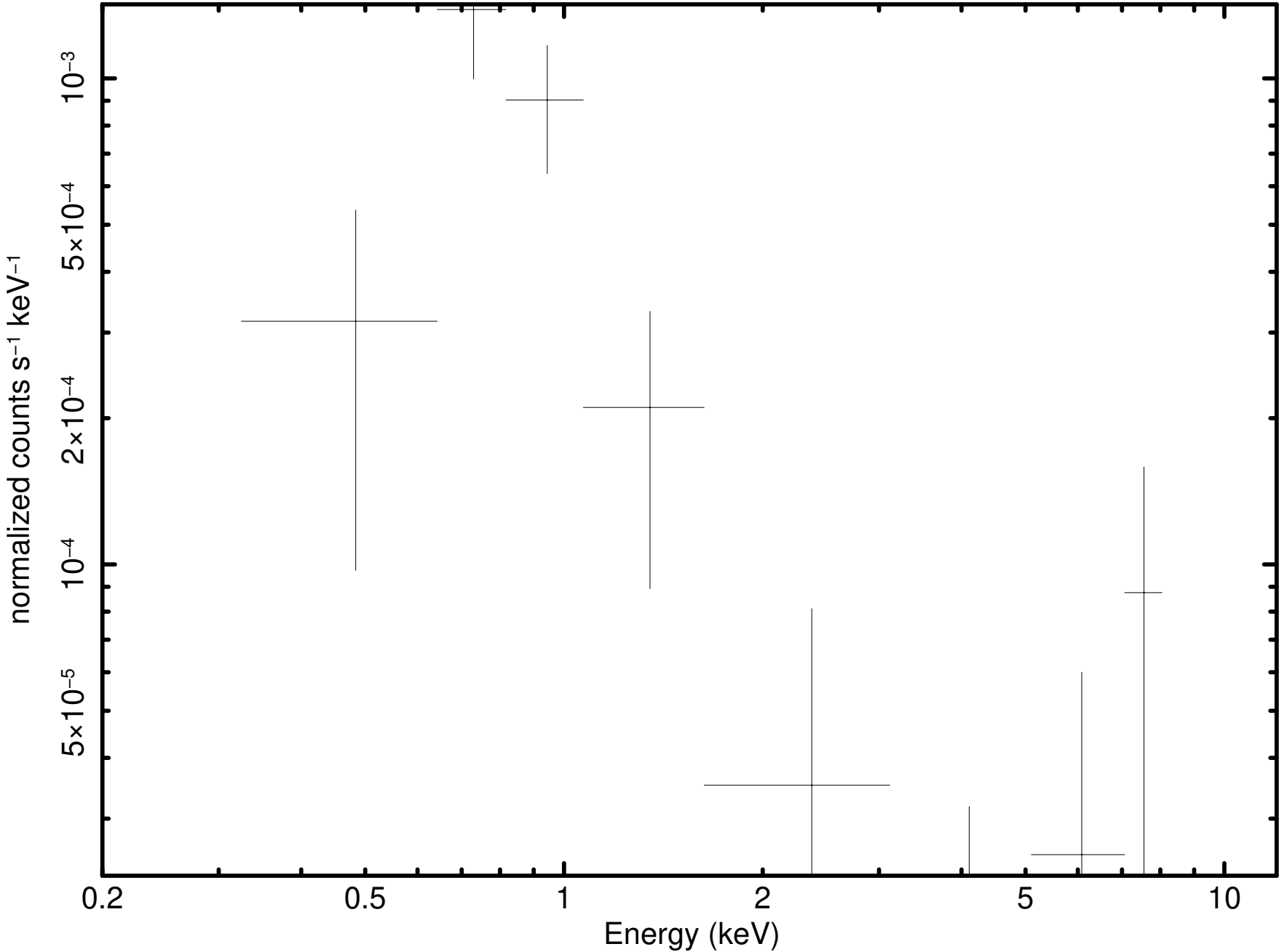
Source 113 minus background (P0931790101PNS003SRSPEC0071)
