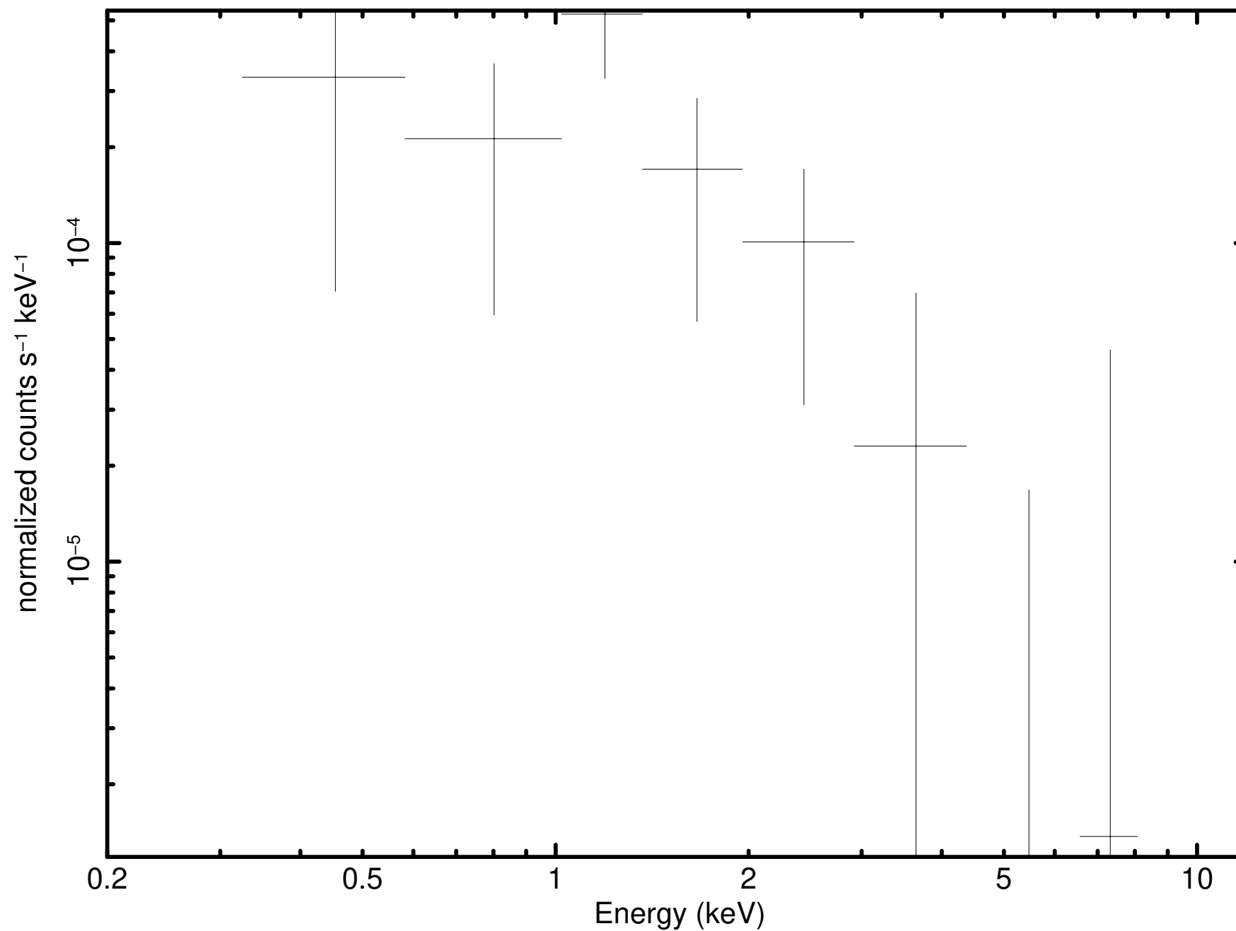
Source 116 minus background (P0931790101PNS003SRSPEC0074)
