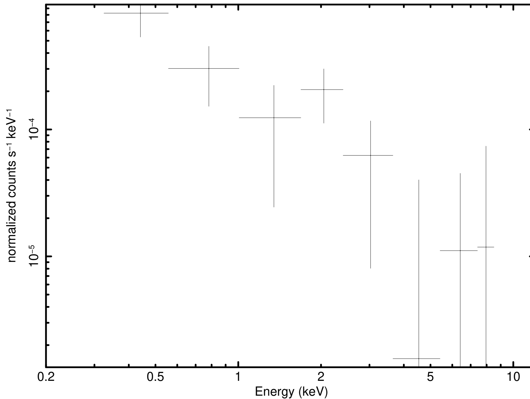
Source 117 minus background (P0931790101PNS003SRSPEC0075)
