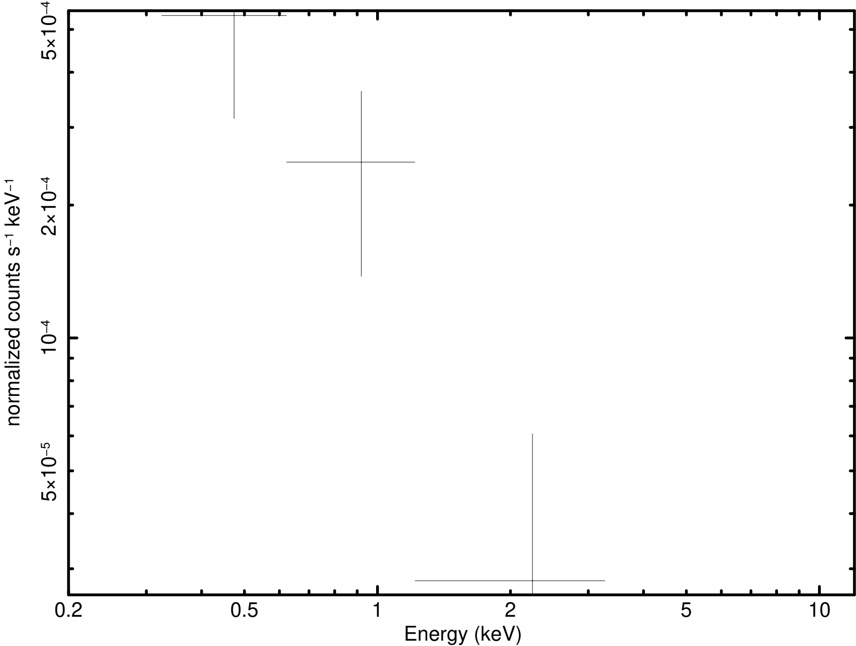
Source 120 minus background (P0931790101PNS003SRSPEC0078)
