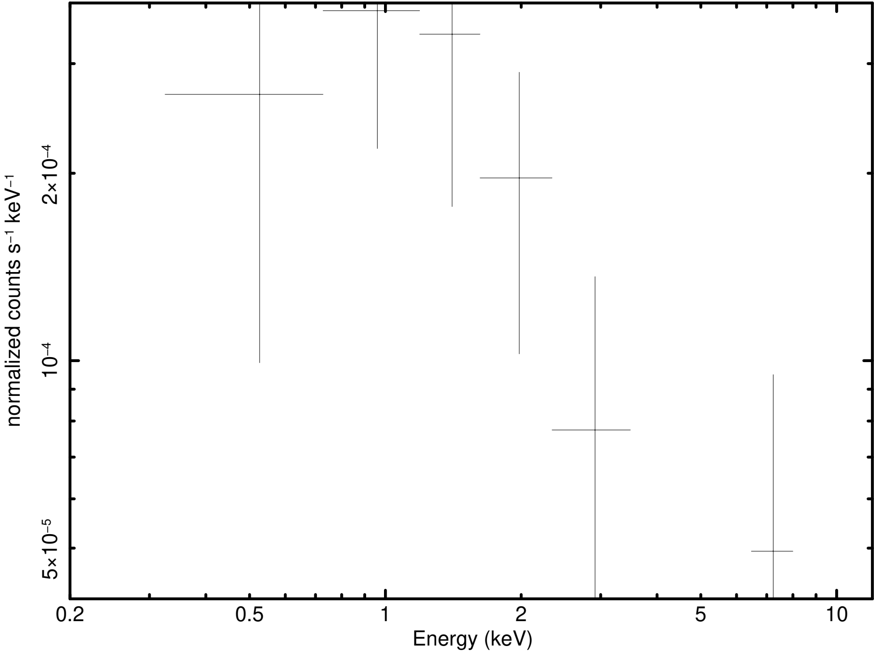
Source 135 minus background (P0931790101PNS003SRSPEC0087)
