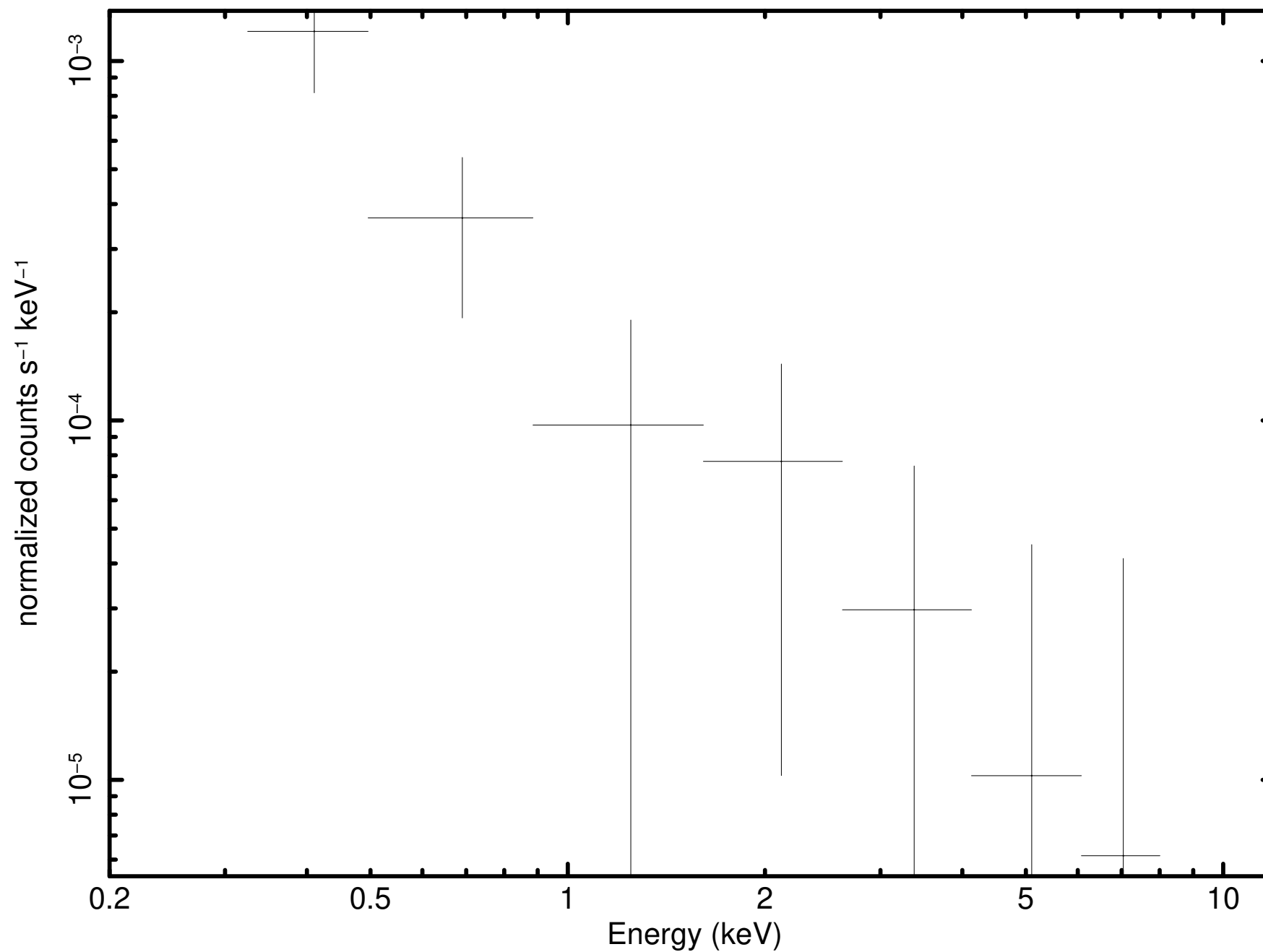
Source 146 minus background (P0931790101PNS003SRSPEC0092)
