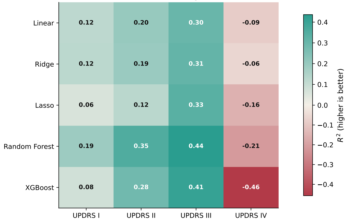
Time-Aware Split
