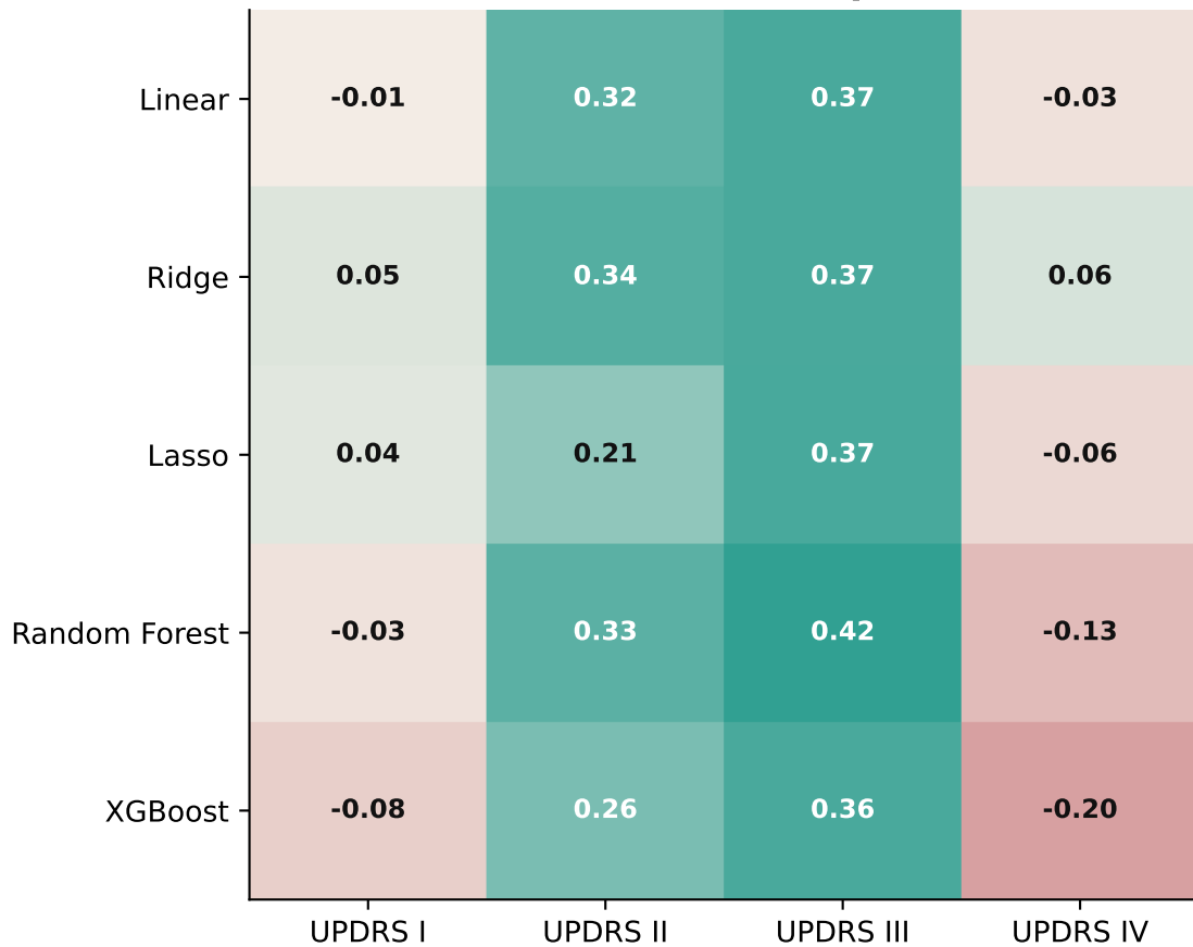
Patient-Level Split
