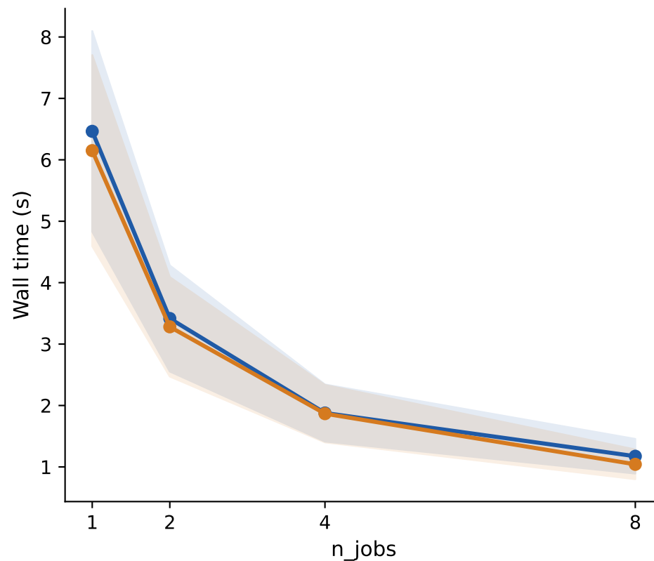
Parallel Scaling on Markov CPU Nodes Random Forest
