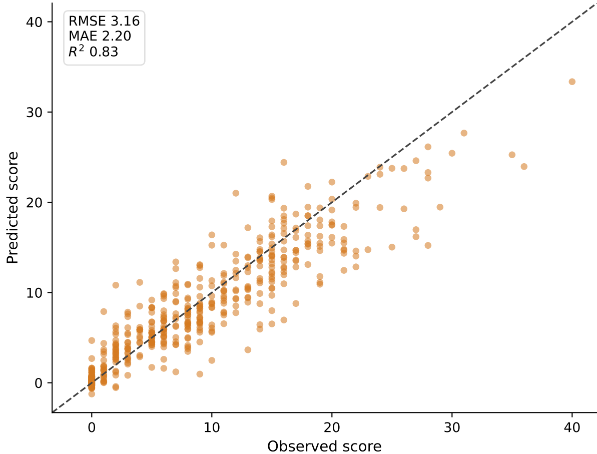
Observed vs Predicted Scores for the Strongest Runs Patient-Level Split Ridge on Future UPDRS III Time-Aware Split Ridge on Future UPDRS II
