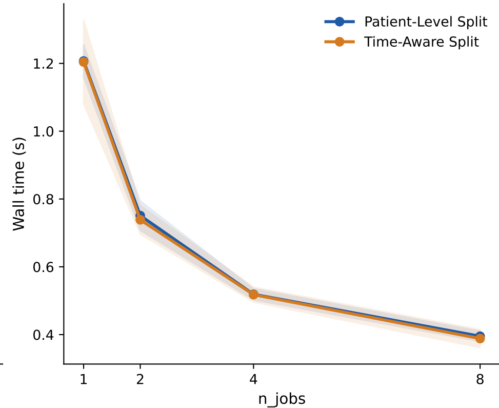
XGBoost
