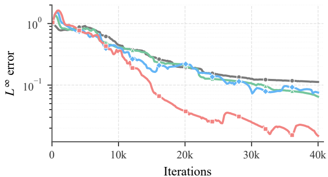
(b) L^\infty error
