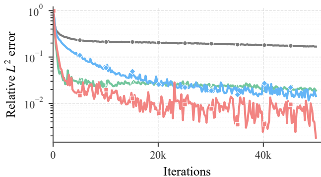
(a) Relative L^2 error
