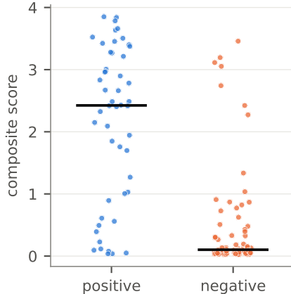
AlphaGenome splicing composite AUC 0.85 (0.77-0.92)
