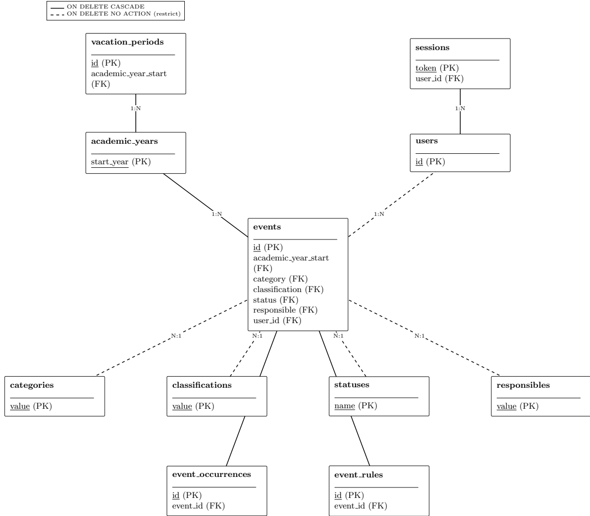
Figure 3.2: Entity-Relationship Diagram, generated from the Drizzle schema. Solid lines are foreign keys with ON DELETE CASCADE ; dashed lines are ON DELETE NO ACTION (the referenced row cannot be deleted while still in use).
