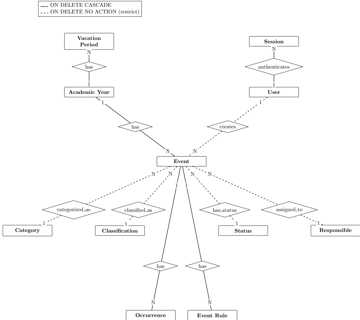
Figure 3.2: Entity-Relationship Diagram, derived from the Drizzle schema.
