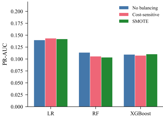
Kaggle-Equivalent (8 features)
