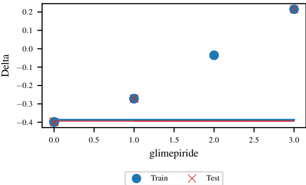
Delta for glimepiride and Class 0
