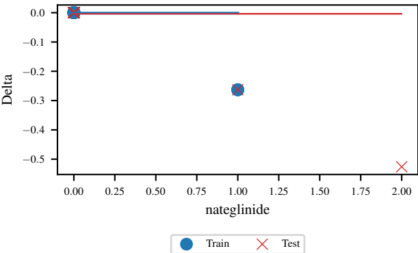
Delta for nateglinide and Class 0
