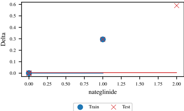
Delta for nateglinide and Class 2
