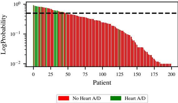
Probability of Heart A/D using KAAM (delta matrix)
