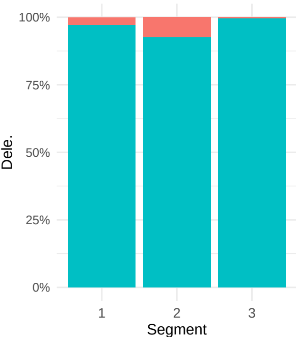
Enrollment Type
