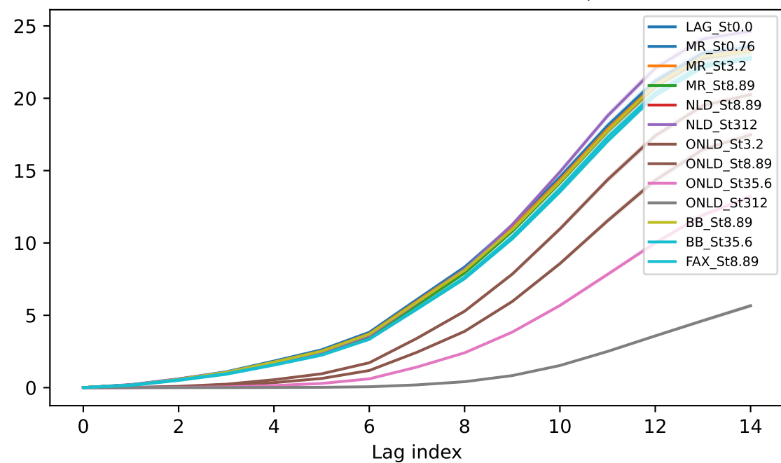
4th-order Structure Function S_4
