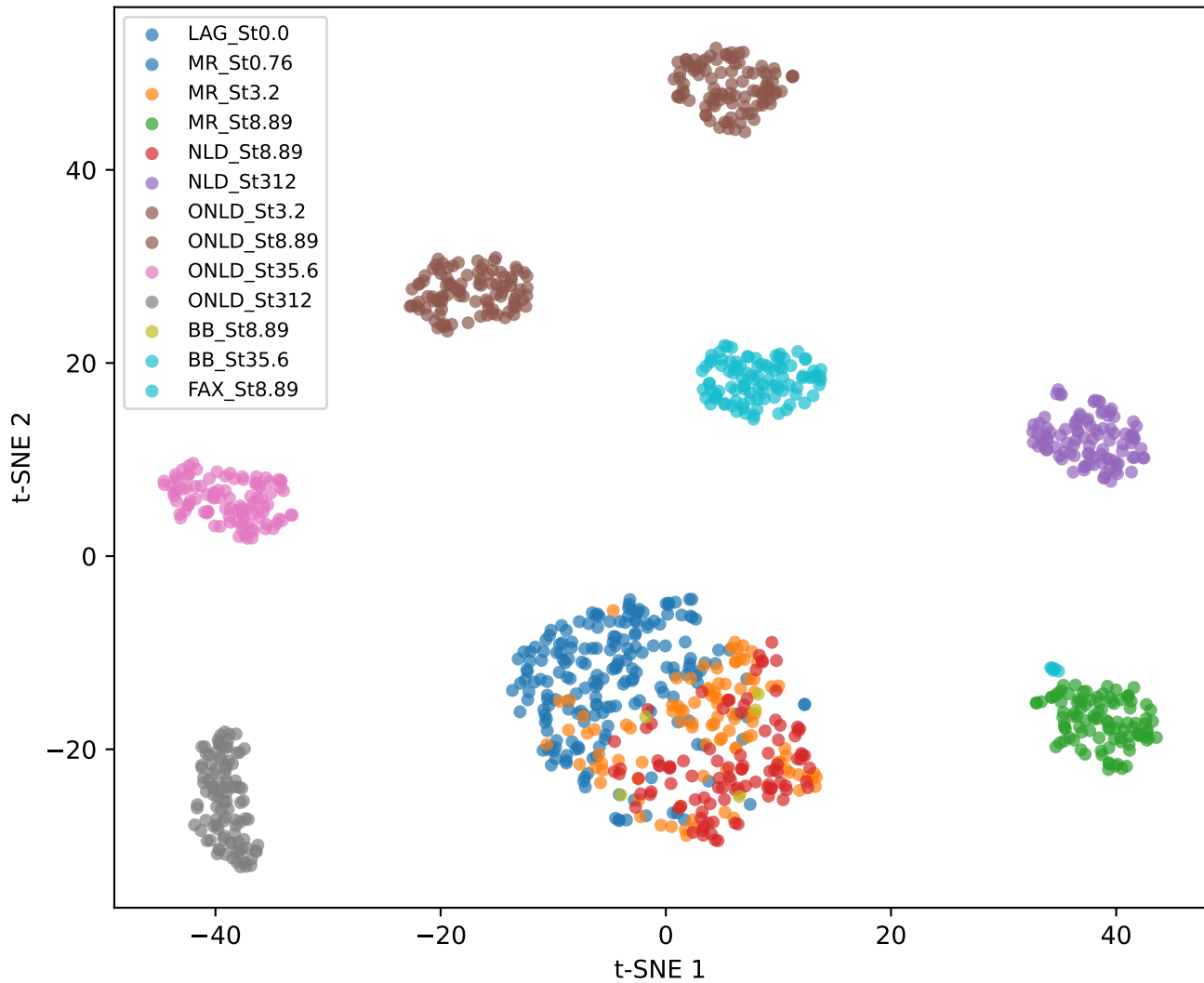
t-SNE (perplexity=30)
