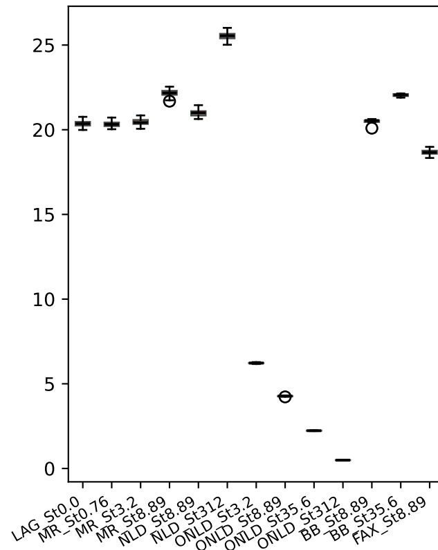
acc variance
