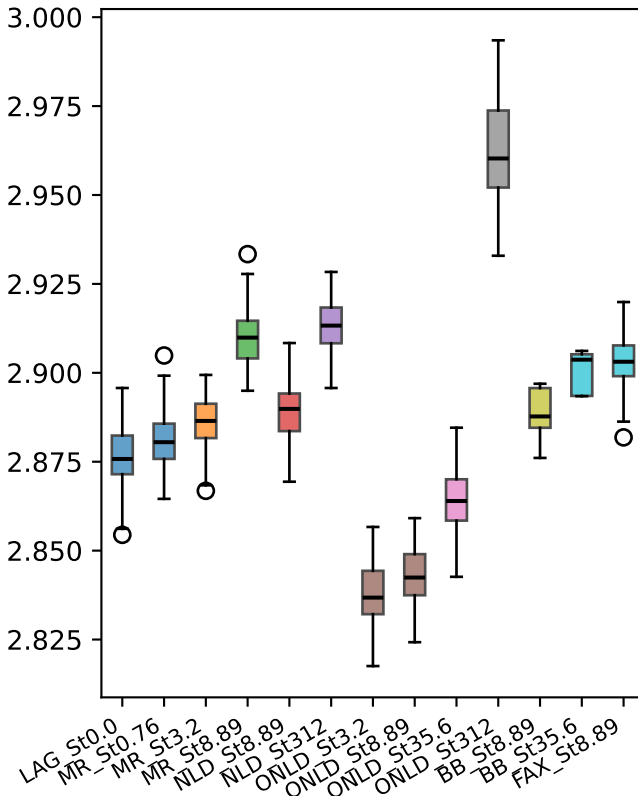
vel kurtosis
