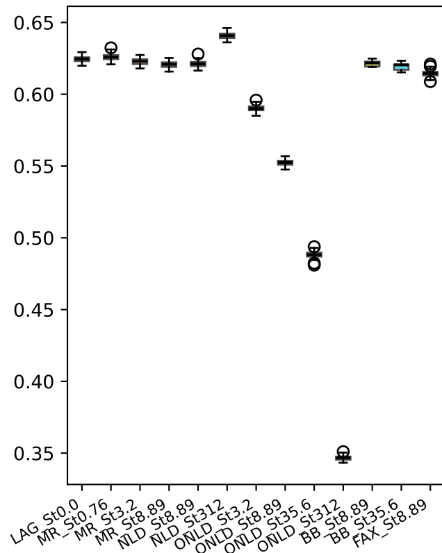
vel variance
