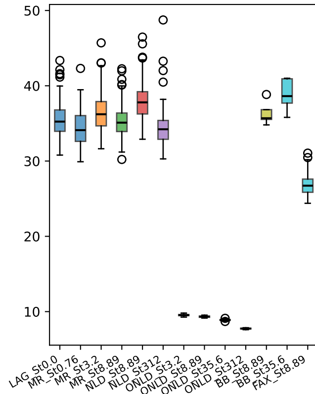
acc flatness
