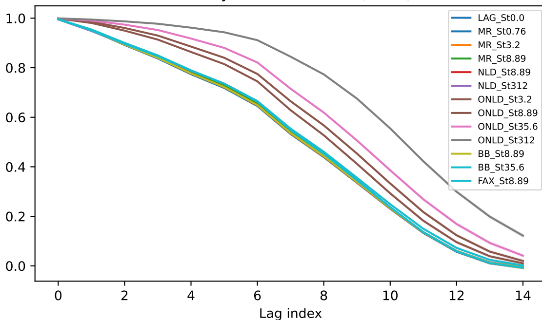
2nd-order Structure Function S_2
