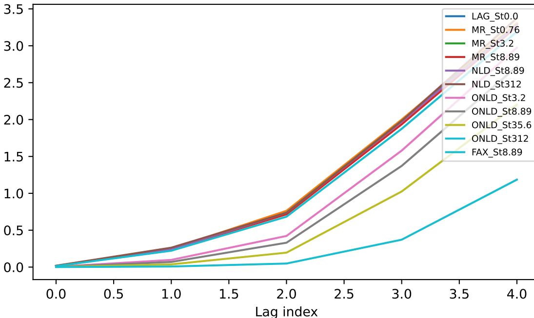
2nd-order Structure Function S_2
