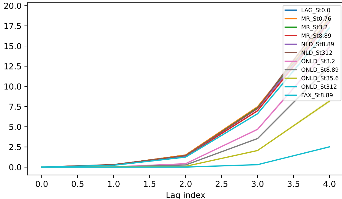
4th-order Structure Function S_4
