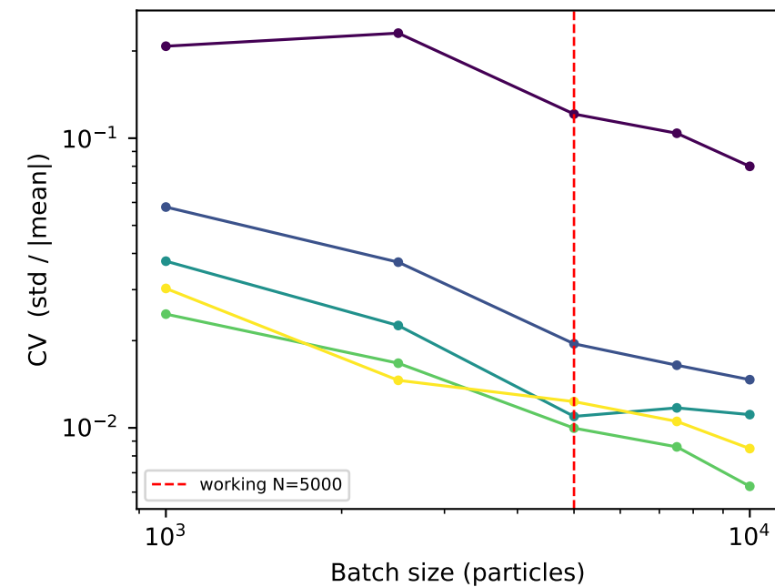
S4 — coefficient of variation vs batch size
