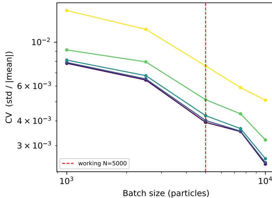
MSD — coefficient of variation vs batch size
