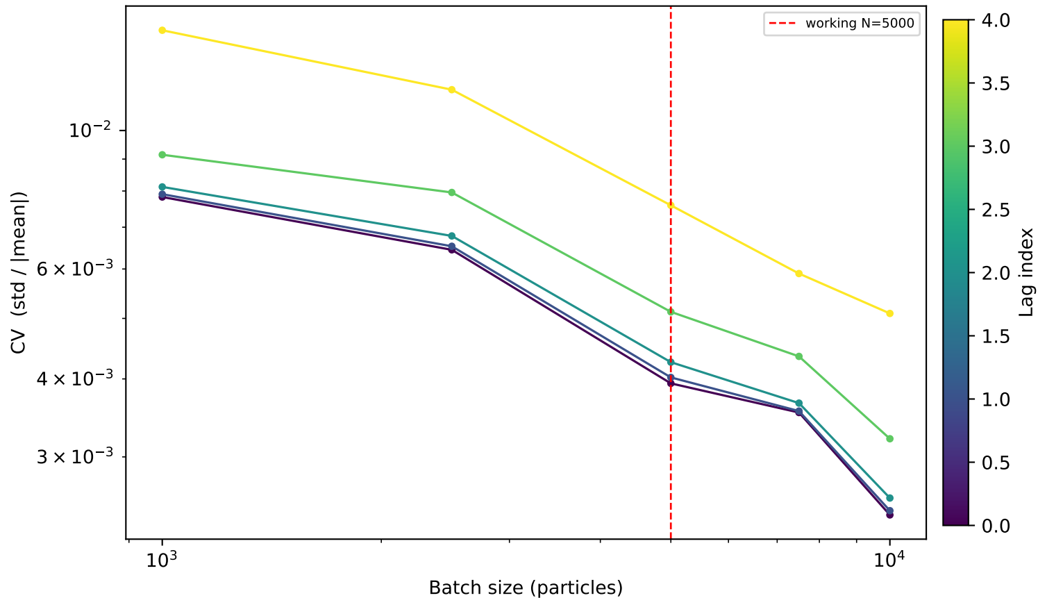
MSD — coefficient of variation vs batch size
