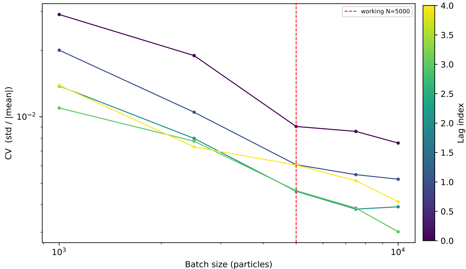
S2 — coefficient of variation vs batch size
