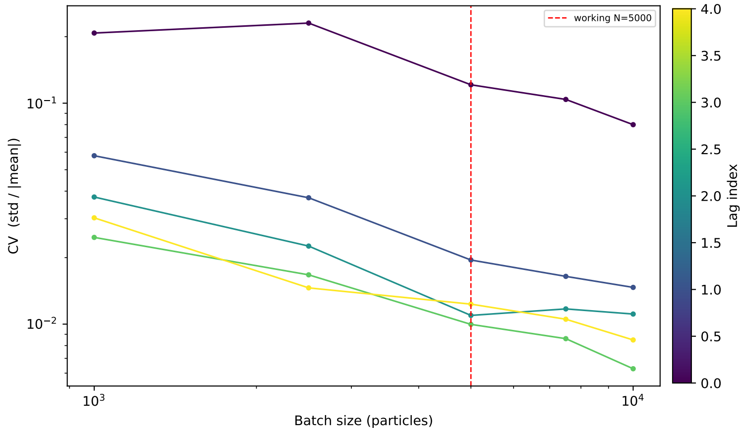
S4 — coefficient of variation vs batch size
