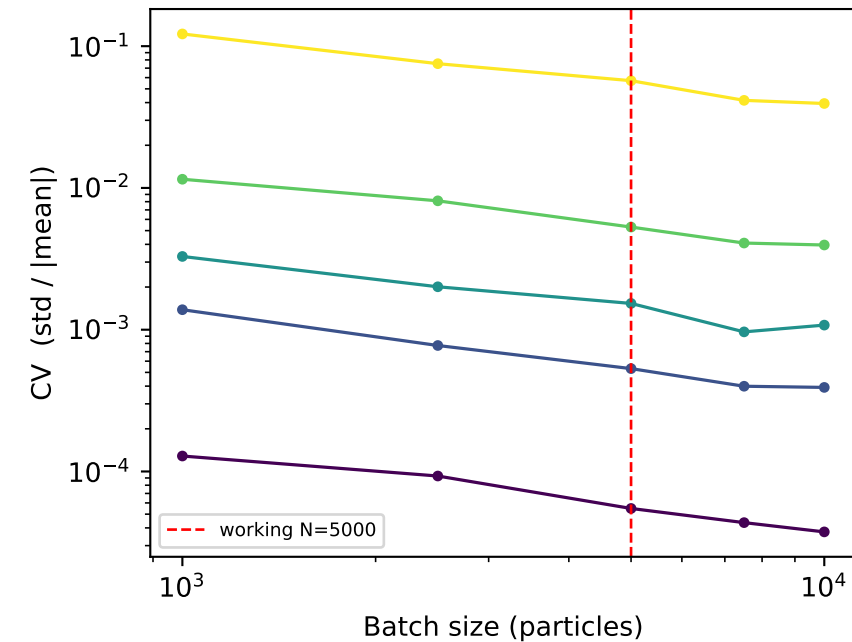
VACF — coefficient of variation vs batch size
