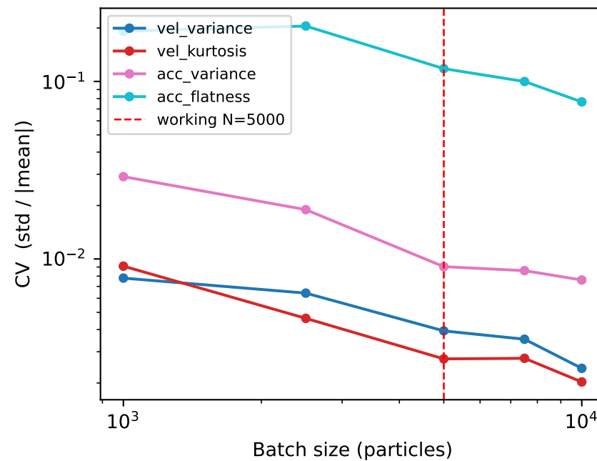
Scalar features
