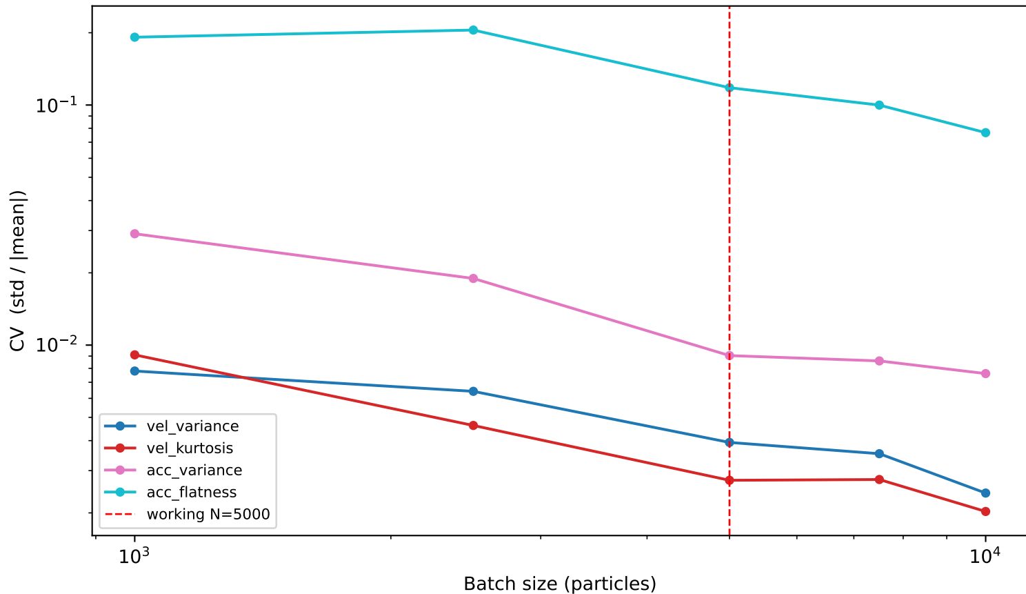
Scalar features
