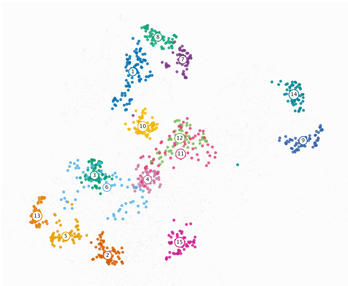
Figure 8: Embedding map of the 15 largest limitation frontier-signal clusters in the 2025–2026 NBER extraction. The clustering input contains 6,196 extracted limitation records from 1,381 papers; 5,575 records had embeddings, 3,991 records were assigned to 129 HDBSCAN clusters, and this figure highlights the largest 15 clusters containing 962 assigned records. Records were routed by extracted constraint family, embedded with OpenAI text-embedding-3-large embeddings, projected with UMAP for display, and clustered with HDBSCAN using the leaf-style frontier-clustering run. Codex (GPT-5.5, extra-high reasoning) reviewed all input text for each displayed cluster before assigning the researcher-facing labels. Colored points show the highlighted largest-15 clusters; grey points are other extracted limitations in the same embedding window. Numbers correspond to Tables 57 and 59. The map is a researcher-facing index to the tables, not the source of the substantive interpretation.
