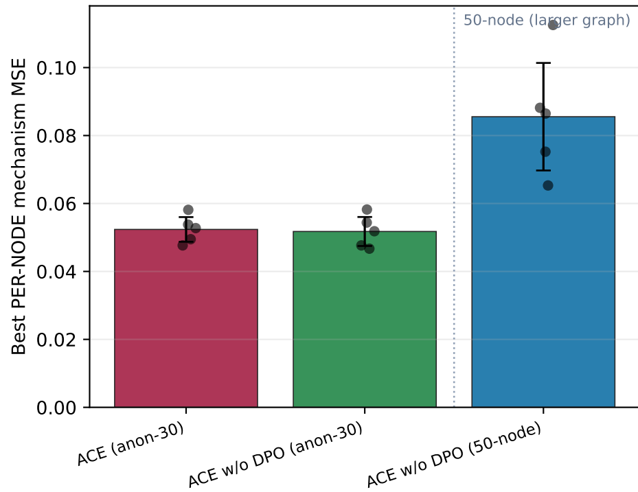
(b) Per-node best MSE (points = seeds)
