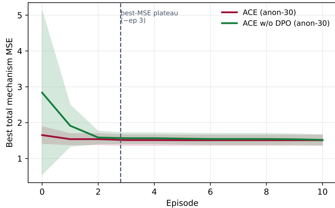
(a) Anonymised 30-node: ACE vs ACE w/o DPO
