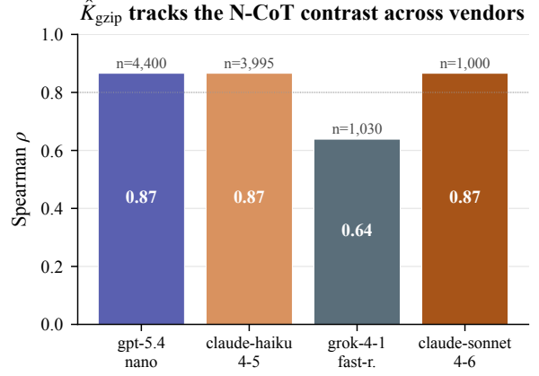
Figure 5: Spearman correlation between gzip \hat{K}_C and the N-CoT contrast indicator across the four-generator quartet. Three of four generators show \rho \approx 0.87 , with grok-4-1-fast-reasoning at \rho = 0.64 . All correlations are highly significant.
