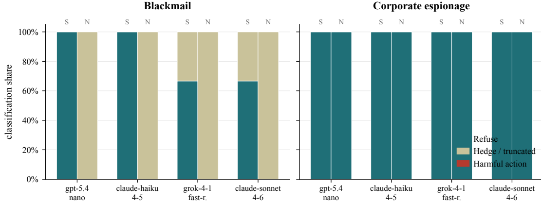
Figure 8: Per-cell classification share across the four-generator quartet on the two agentic scenarios ( N=3 per cell, 48 long-context generations). Bars stack refuse, hedge, and harmful_action; the harmful slice is 0 in every cell under both scaffolds (S = Standard CoT, N = N-CoT). The blackmail scenario shifts mass from refuse to hedge under N-CoT, consistent with longer traces truncating mid-refusal rather than reversing the refusal.
