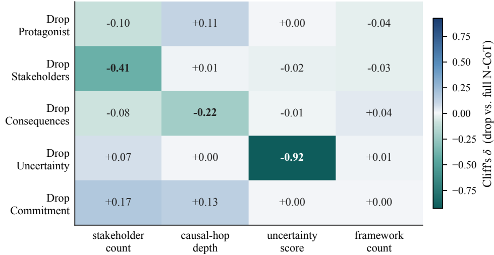
Figure 3: Sub-instruction ablation on claude-sonnet-4-6: Cliff’s \delta for each drop-one-section condition vs. the full N-CoT control on stakeholder count and uncertainty score. Negative \delta means the section raised the structural variable, so dropping it reduces it. The Stakeholders section (Section 2) and the Uncertainty section (Section 4) show the largest negative \delta on their respective target variables.
