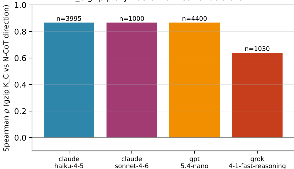
K_C gzip proxy tracks the N-CoT structural shift
