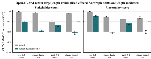
Figure 3: Tier-1 Cliff’s \delta effect sizes (N-CoT vs. standard CoT) on the four structural variables, with bootstrap 95% CIs. All four generators show large positive \delta s on stakeholder count and uncertainty score ; effect sizes are robust to length residualisation on the OpenAI and xAI generators, while shrinking toward zero on the two Anthropic generators.
