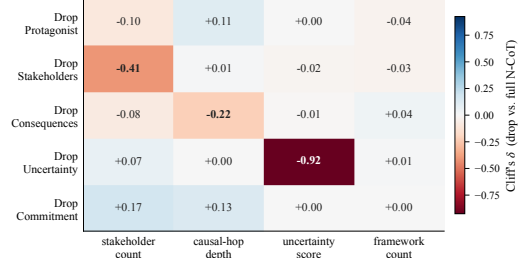
Each substantive section carries its target metric (claude-sonnet-4-6, N=3 , 30 scenarios)
