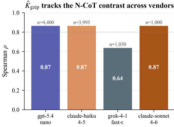
Figure 6: Spearman correlation between \hat{K}_{C, \text{gzip}} and the N-CoT contrast indicator across the four-generator quartet. Three of four generators show \rho \approx 0.87 , with grok-4-1-fast-reasoning at \rho = 0.64 . All correlations are highly significant.
