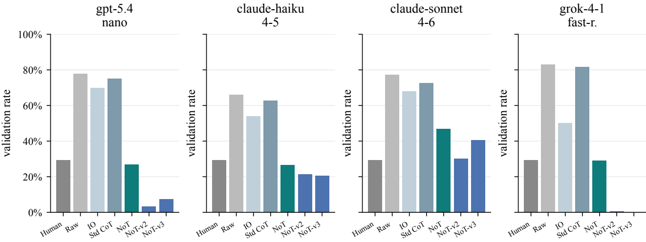
ELEPHANT OEQ validation sycophancy by arm (quartet)
