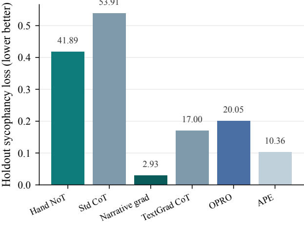
Phase 14: optimizer comparison on OEQ holdout
